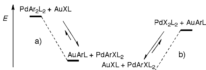
Figure 2. Qualitative thermodynamic balances for arylation exchange between gold Au I and Pd II complexes.
