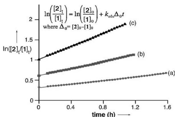
Figure 3. Plot of \ln([2]_t/[1]_t) versus time: a) [2]_0 = 0.014 \text{ mol L}^{-1} ; b) [2]_0 = 0.019 \text{ mol L}^{-1} ; c) [2]_0 = 0.028 \text{ mol L}^{-1} . Starting conditions: [1]_0 = 0.01 \text{ M} in THF at -10^\circ\text{C} .
